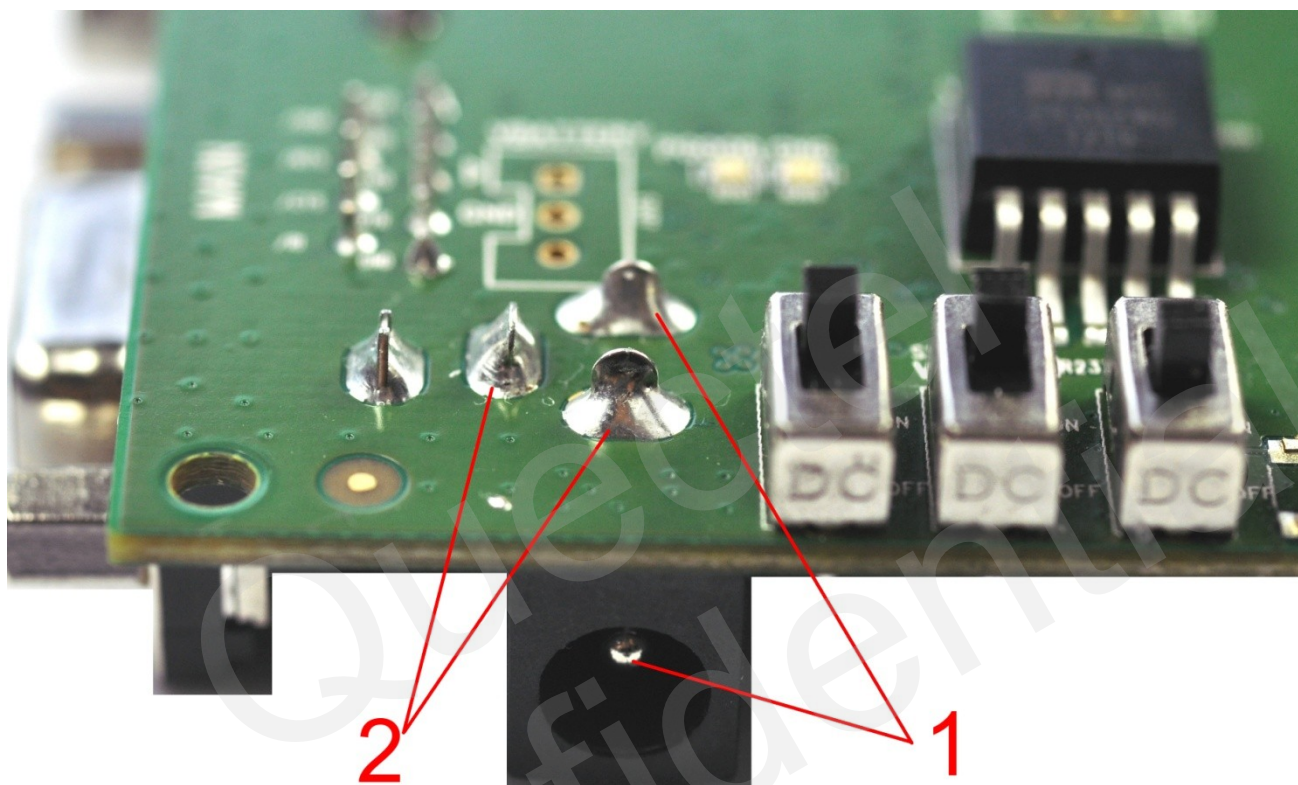
Figure 4: Power interface
