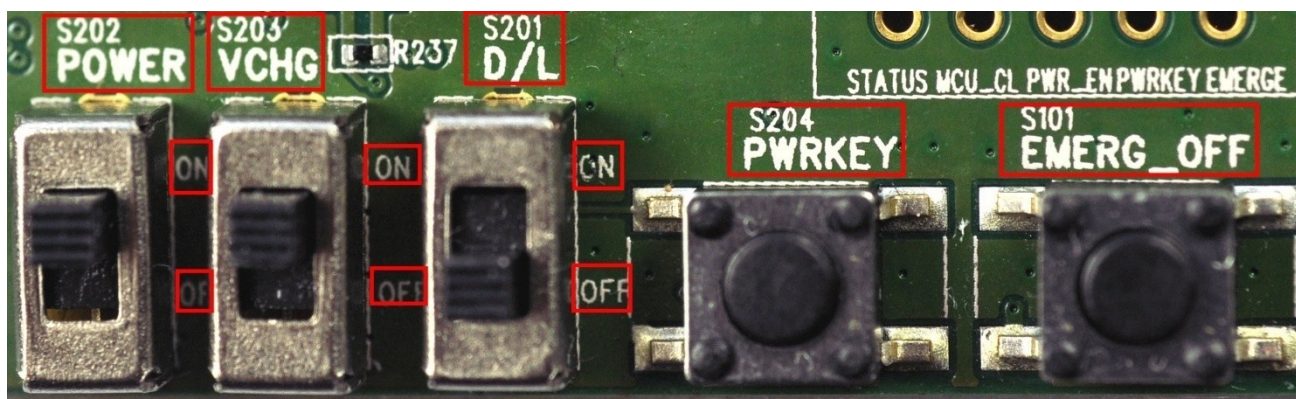
Figure 10: Switch
