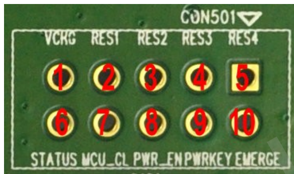
Figure 16: CON501 points
