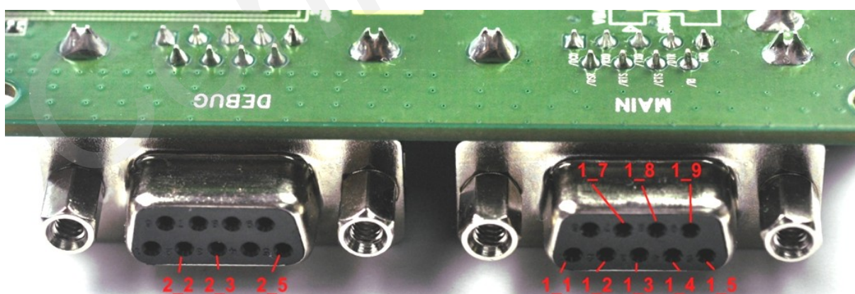
Figure 8: Main port and Debug port
