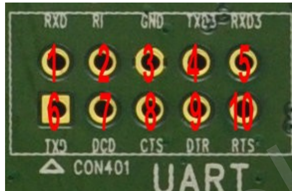
Figure 15: CON401 points
