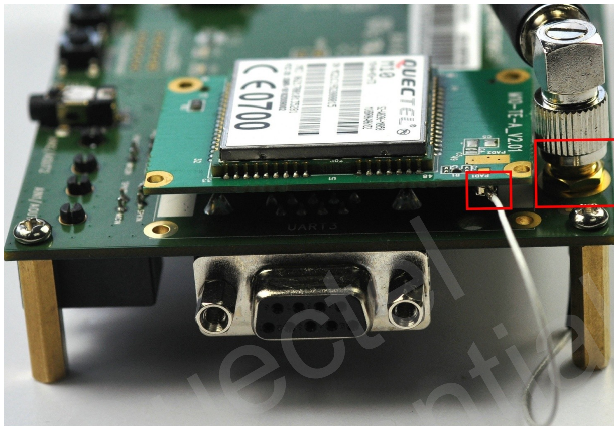
Figure 7: Antenna interface
