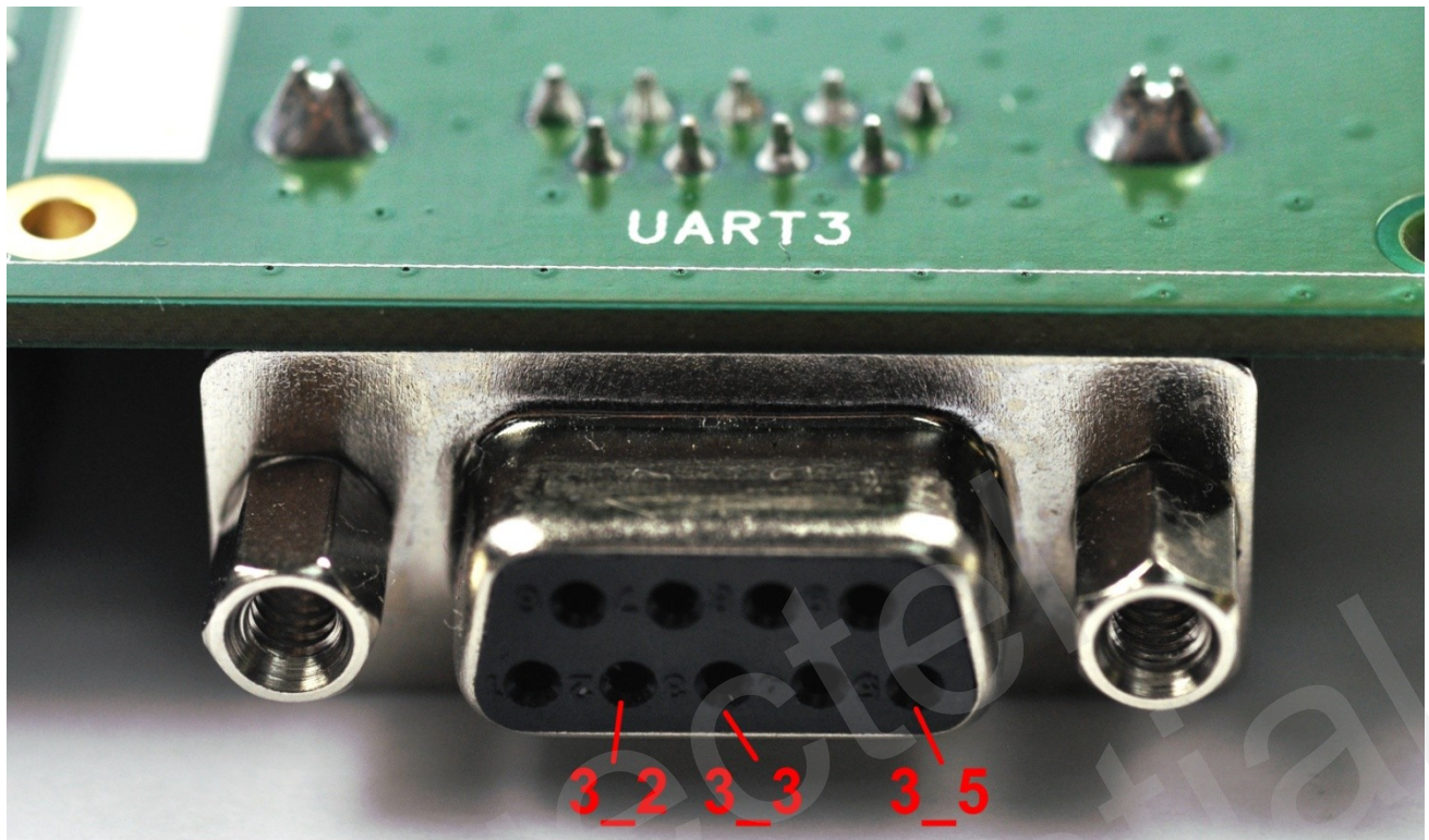
Figure 9: UART3
