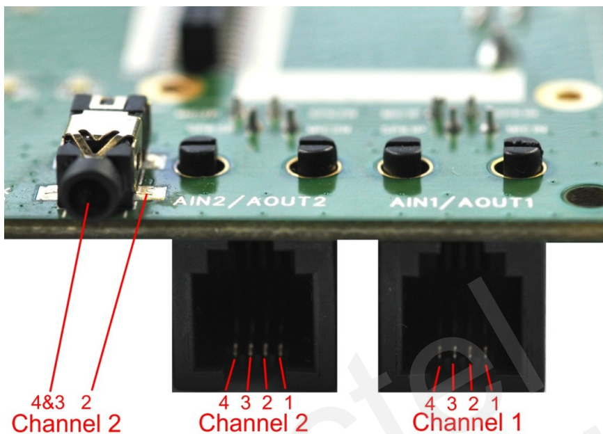
Figure 5: Audio interface
